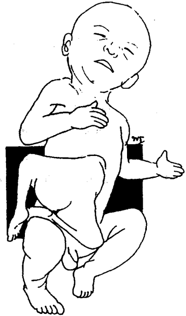
Figure 14. Parasite fetus.
