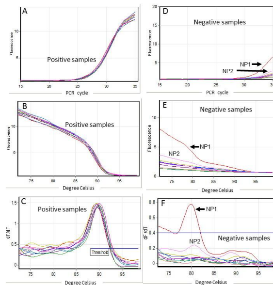
Figure 4 Sensitivity and specificity of SYBR® green real-time PCR and melt curve analysis for chromosome 1 detection. (A-C) Positive samples. (D-F) Negative samples. (A and D) PCR fluorescence pattern during PCR reaction, PCR products were raised before 25 cycles whereas nonspecific product (NP) were raised after 30 cycles. (B and E) Post PCR melt fluorescence pattern. (C and F) Melt curve analysis, the melt peak of PCR products ranged from 88 to 90°C and the threshold for df/dt unit of melt curve was 0.4. The melt peak of primer dimer is 80°C. NP1 represents samples with high amount of nonspecific products while NP2 represents samples with small amount of nonspecific products
