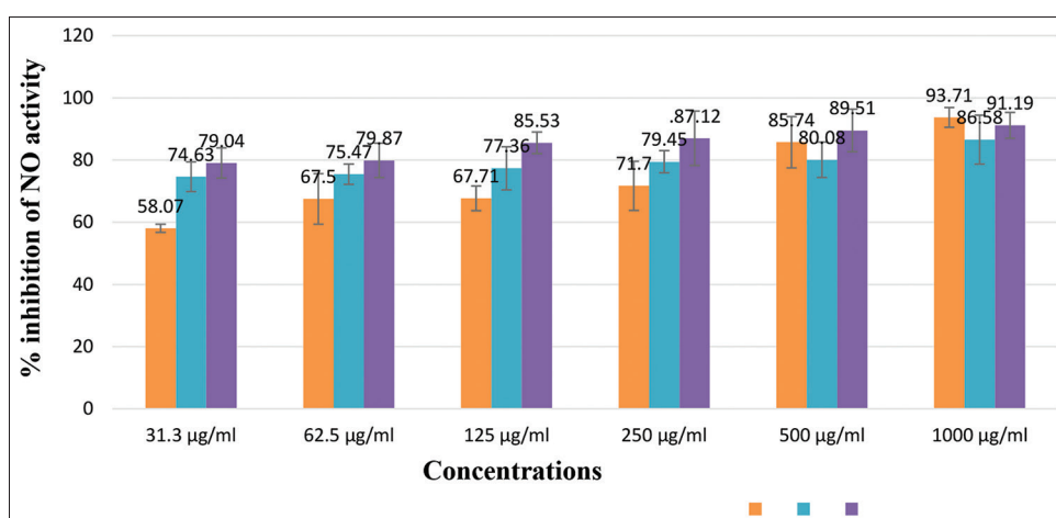
Figure 3: Nitric oxide scavenging activity of MFBB (orange) and CFBB (aqua) ascorbic acid (purple). Inhibition of NO activity increased in a concentration-dependent manner with methanol extract having the highest inhibition (93.71%) at 1000 µg/ml. Values are expressed in % ( n = 3 , triplicate)
