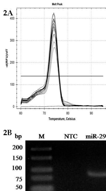
Figure 2 Melting curve analysis of PCR products revealed a specific product ( T_m = 74^\circ\text{C} ), which was related to the expected amplicon size of miR-29a (Fig 2a). PCR products were run on low melting agarose gel 5% Nuseive 3 : 1 agarose gel (M: 10 bp DNA marker, NTC: no template control, PCR products of miR-29a).
