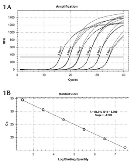
Figure 1 Standard curve for ten-fold serial dilutions of pGEM-miR29a. Amplification plots of qRT-PCR with DNA template from plasmid (pGEM-miR29a) with ten-fold serial dilution ( 2.99 \times 10^7 , 2.99 \times 10^6 , 2.99 \times 10^5 , 2.99 \times 10^4 , 2.99 \times 10^3 , 2.99 \times 10^2 copy number). C_q values were plotted against corresponding log concentration (Fig 1a). Slope of standard curve was -3.700 and R^2 was 1.00 with 86.3% efficiency (Fig 1b).
