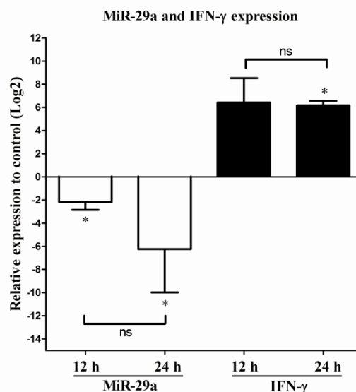
Figure 3 Expression of pri-miR-29a and IFN- \gamma in Con A treated PBMCs. 5 \times 10^5 PBMCs isolated from three individual pigs were incubated with Con A at 10 \mu\text{g}/\text{ml} for 12 and 24 hours. Expression of pri-miR-29a and IFN- \gamma in Con A stimulated PBMCs were measured by qRT-PCR. \log_2 value represents relative expression level compared to untreated control cells at each time point. * : p < 0.05 and ns : not statistically significant.
