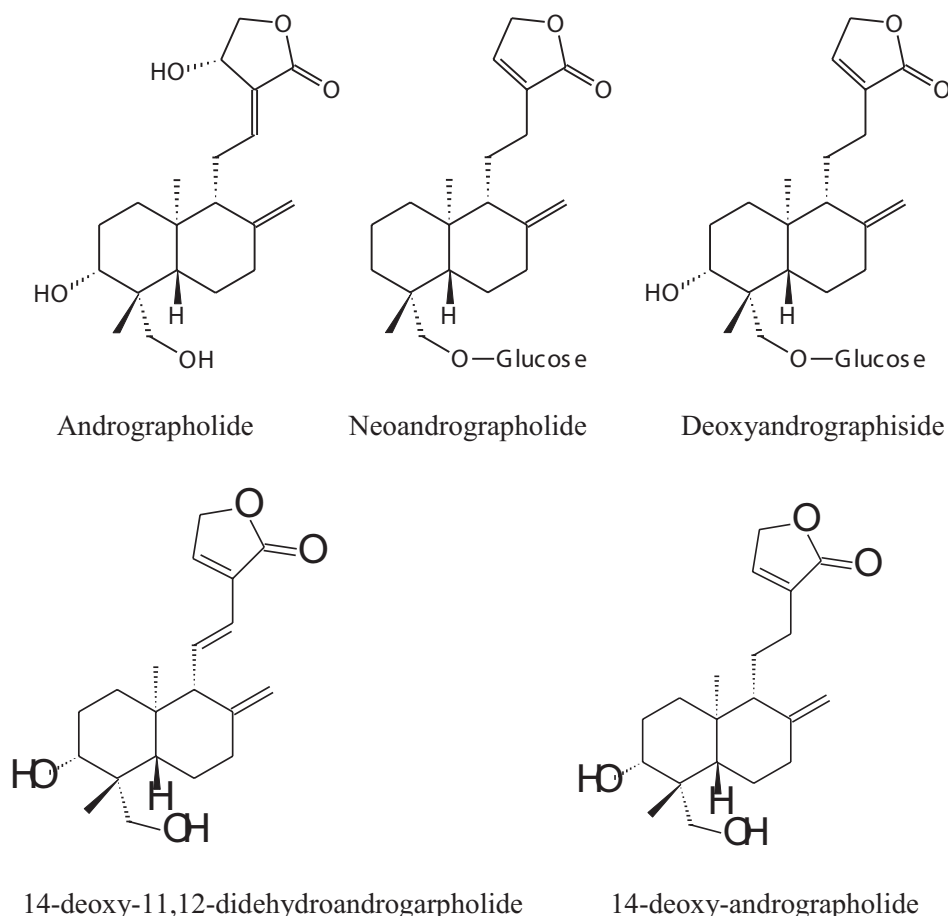
Figure 1: Chemical structures of andrographolide, neoandrographolide, deoxyandrographiside, 14-deoxyandrographolide, and 14-deoxy-11,12-didehydroandrographolide
