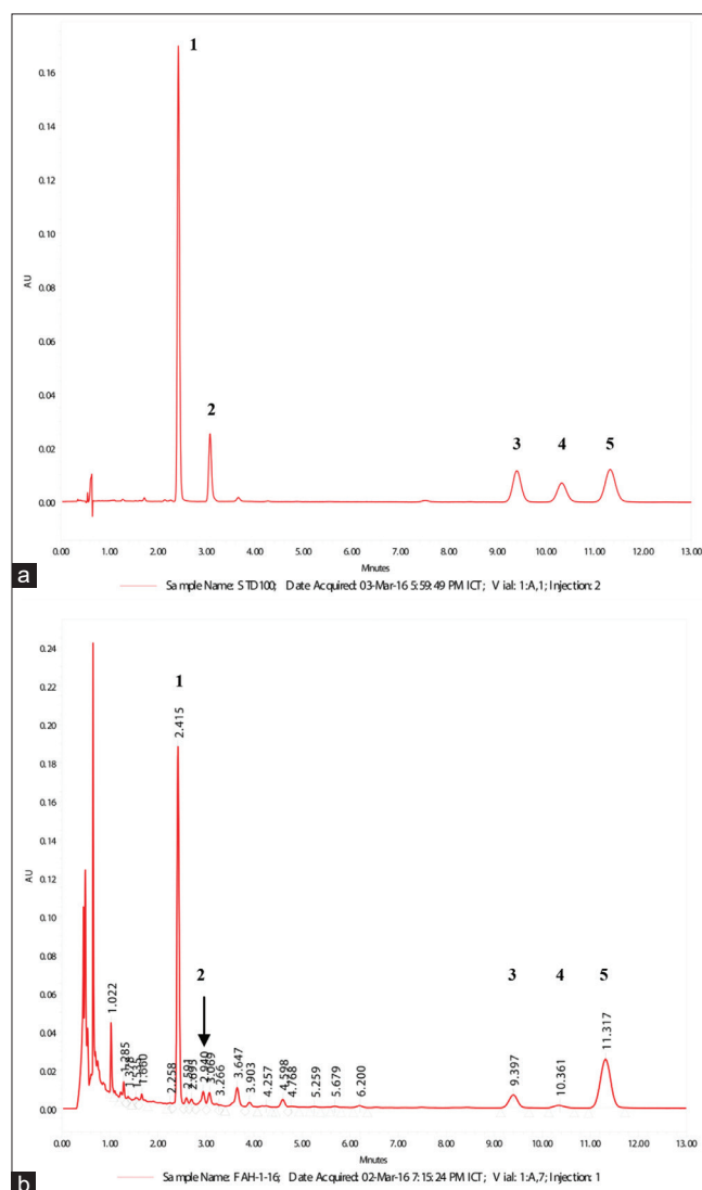
Figure 2: UPLC chromatograms of (a) standard mixing solution at concentration of 100 \mu\text{g}/\text{ml} and (b) sample solution. Peaks; 1: Andrographolide, 2: Deoxyandrographiside, 3: Neoandrographolide, 4: 14-deoxyandrographolide and 5: 14-deoxy-11,12-didehydroandrographolide
