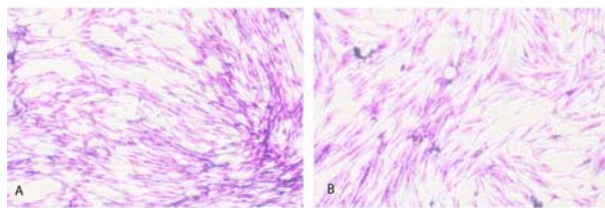
Figure 3 Spindle-shaped morphology of BM-MSCs (A) and AD-MSCs (B) at day 10.
