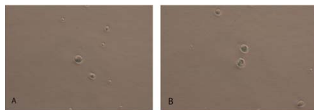
Figure 1 Adherent MNCs at day 1 post-plating. Cells derived from both BM (A) and AD (B) showed similar morphology with heterogeneity in cell size; \times 400 .
