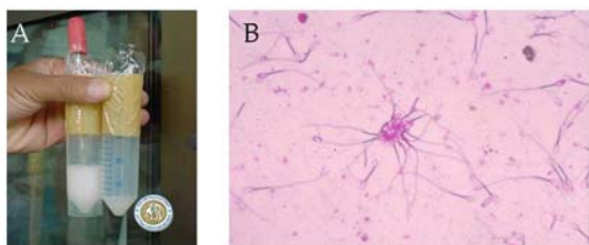
Figure 2. (A) Asian elephant ( Elephas maximus ) fresh semen collected by manual rectal stimulation (B) Asian elephant spermatozoa stained with Eosin-Nigrosin dye.
